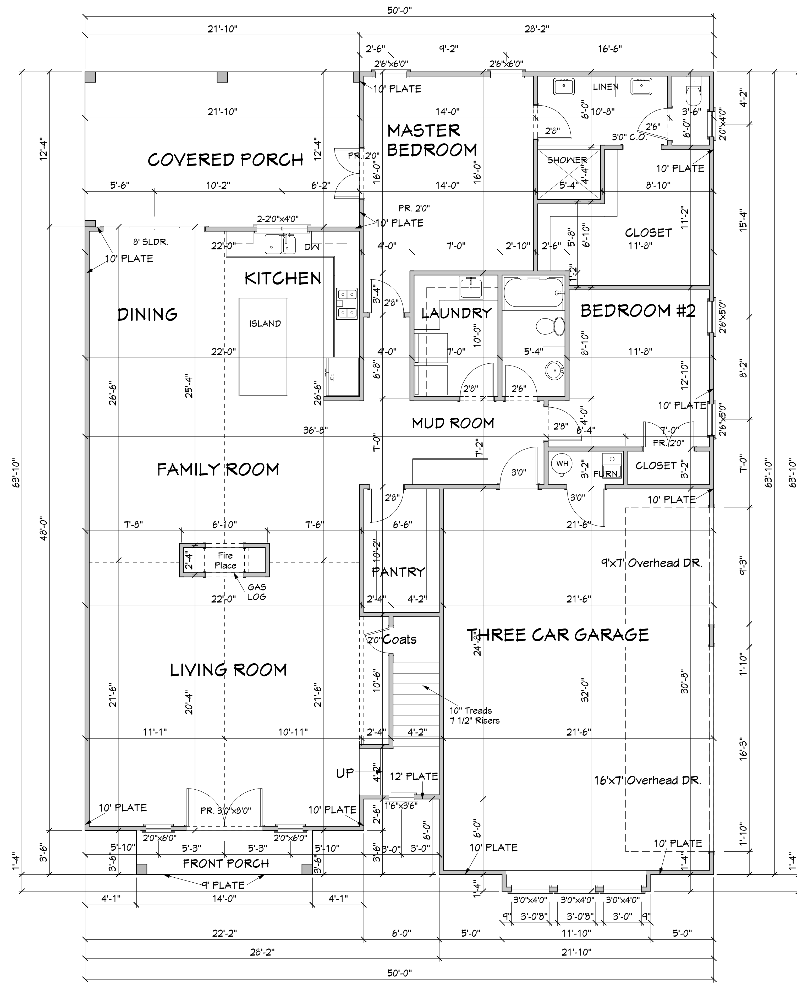
MAIN LEVEL 2,104 S.F. 1/4"=1'-0"
